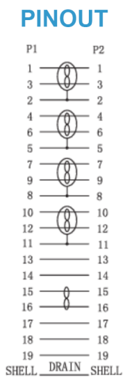
HDMI A male
